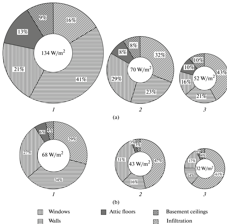
Fig. 5. The structure of heat losses in individual (two-storied) buildings (a) and in apartment (nine-storied) buildings (b) (at t_{\text{out}} under conditions of Moscow). Notations see Fig. 4.
