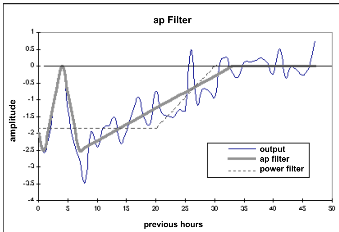
Fig. 9. Filter obtained for ap index.
