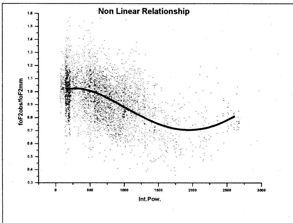
Fig. 3. Non-linear relationship between the ionospheric response ( \Phi ) and the integral of the auroral power.
